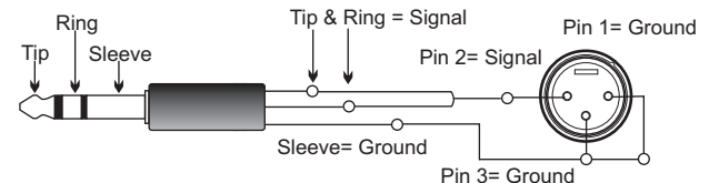
Special Adaptor TRS/XLR to use a console insert as direct output
